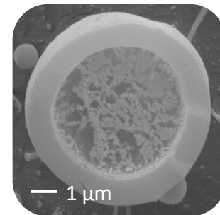
Scanning electron microscopy image of PAD™ droplet
